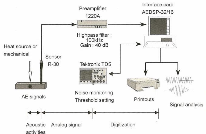
Fig. 1. Diagram of the acoustic emission detection system.
