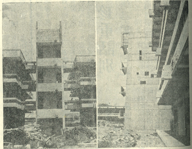
實為翼右，棟室驗實生學為翼左其，樓塔形矩的霄雲入臨 。棟室究研及備準驗
