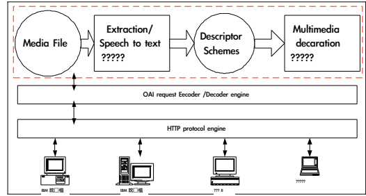
Figure 1. Framework of Open Archive Initiative protocol
