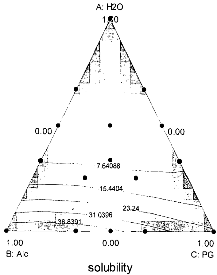
Fig 1: Contour plot of oxatomide solubility (mg/ml) in the solvent mixture containing water, alcohol and propylene glycol.
