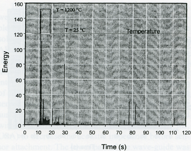
Fig. 5. Acoustic emission energy for the 1200 °C group with pure powder flux during the soldering period.
