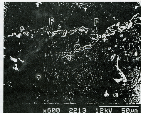
Fig. 7. Crack (C) propagating along the flux inclusions (F) from the longitudinal surface of specimens at the soldered area.
