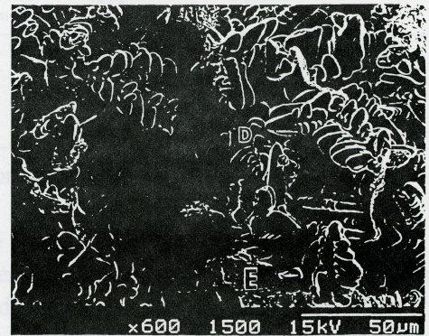
Fig. 6. Surface of a fractured specimen showing the dendritic crystallized structure (D) and equiaxial grains (E) of the parental metal (6a) soldered at 1200 °C and (6b) 1150 °C.
